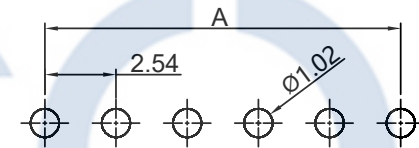
Recommended P.C.Board Hole Layout (Tolerance:±0.05)
