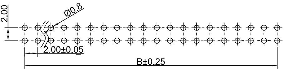
SUGGESTED PCB LAYOUT (COMPONENT SIDE)
