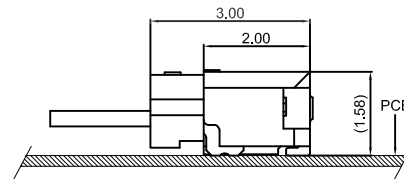
Mated Condition
