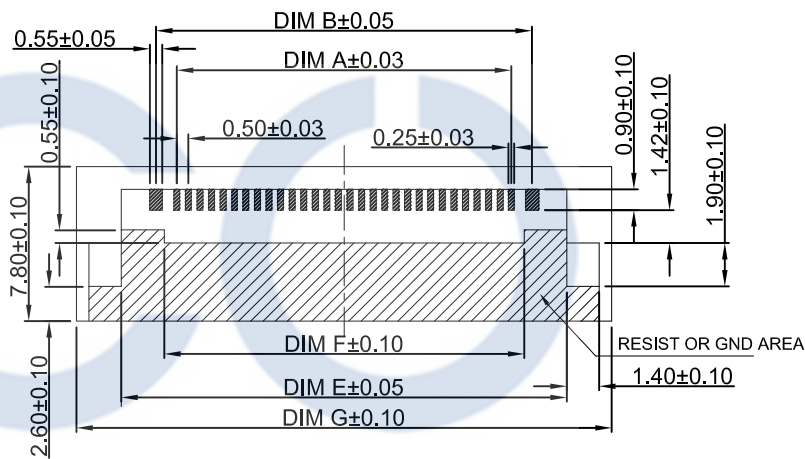
Applicable PCB dimensions
