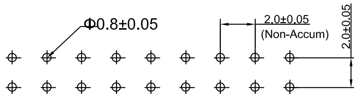
SUGGESTED PCB LAYOUT (COMPONENT SIDE)
