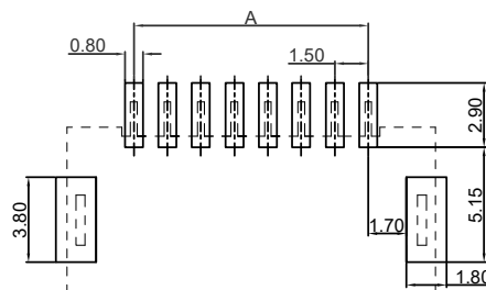
PCB LAYOUT(Tolerance:±0.05)
